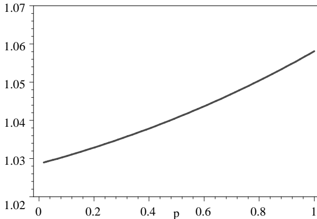
Figure 2: Short-run expected return as a function of p
