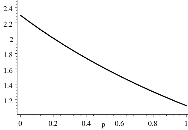
Figure 3: Long-run expected return as a function of p
